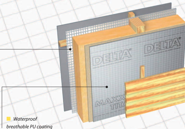
DELTA®-MAXX TITAN for outer-wall insulation
