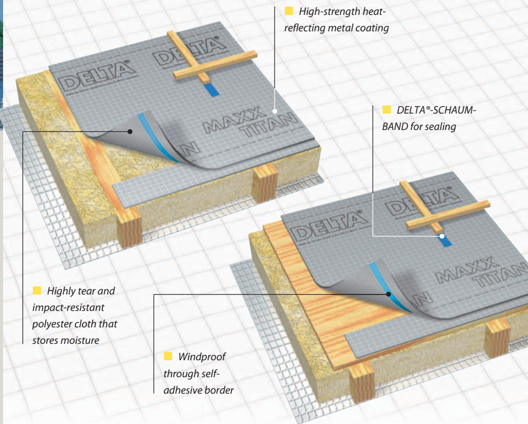
DELTA®-MAXX TITAN for waterproofing and soft sheathing
